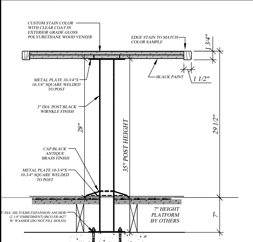
H SECTION
