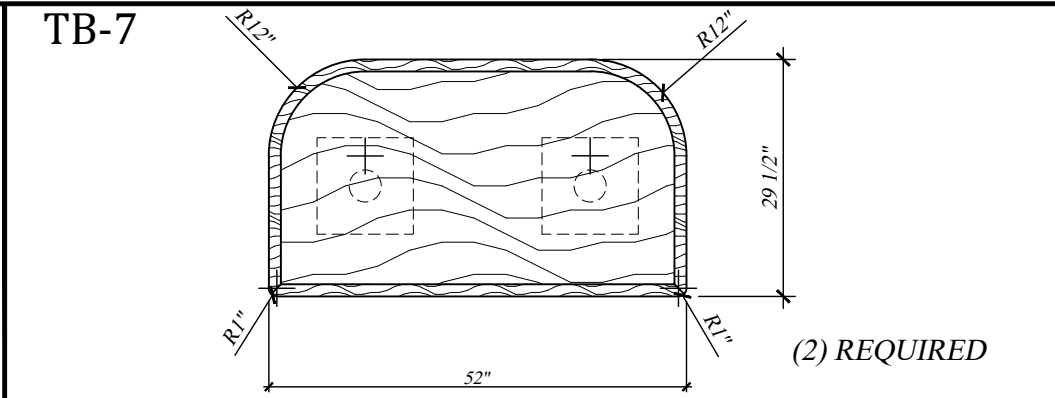
~ FLOOR PLAN SCALE: 1/2"=1'-00"
