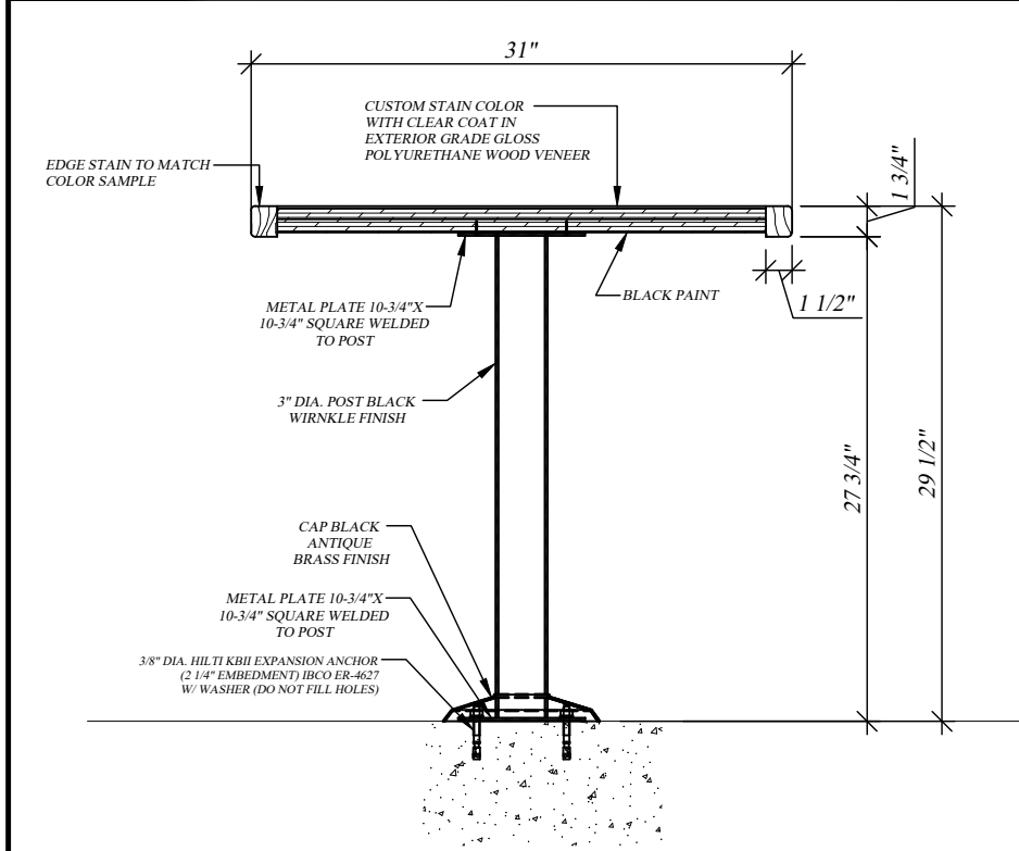
N SECTION
