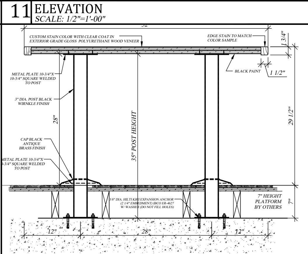
L SECTION
